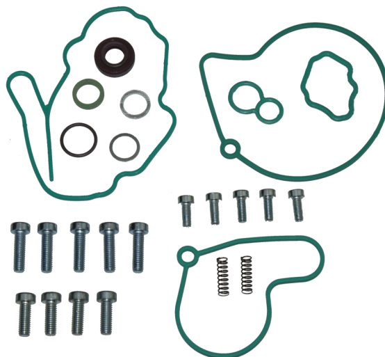
Tandem pump kit for F009D00001, fits Audi/VW
