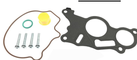
Tandem pump kit for 03L145100F, 03L145100G fits Audi/VW
