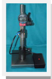
50D259 Ball Cup Movement Measuring Stand & Gauge (More Details Page 33)
