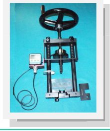
45D0701 Injector & EUI Stripping/Assembly Jig (More Details Page 32)
